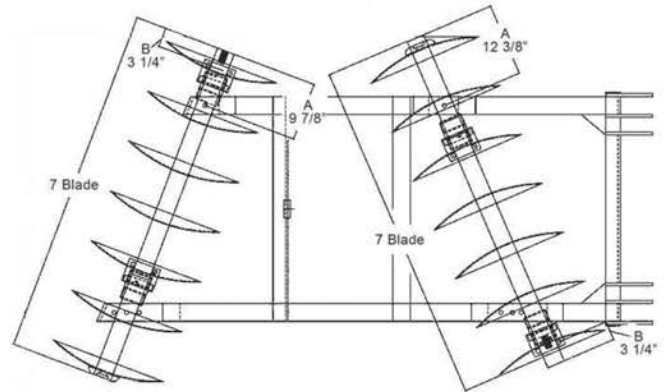
15668 REAR GANG BEAM 3" X 3" X 1/4" SQ. TUBE X 60"
